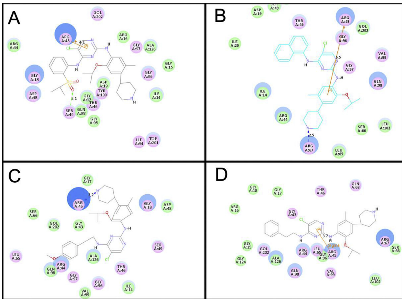
Fig. 6. 2D model of the interactions between amino acid residues and ligands with different bond types and lengths. A) Ceritinib, B) 16j , C) 16d , D) 16c .
