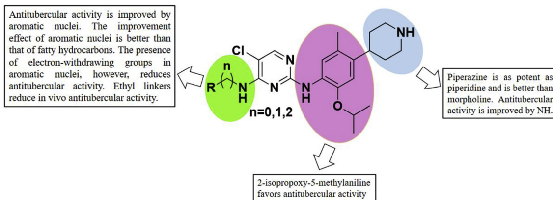
Fig. 4. Structure–activity relationship.
