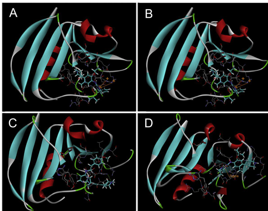
Fig. 5. 3D model of ligands bonded with the active site of the Mtb DHFR enzyme. A) Ceritinib, B) 16j , C) 16d , and D) 16c .
