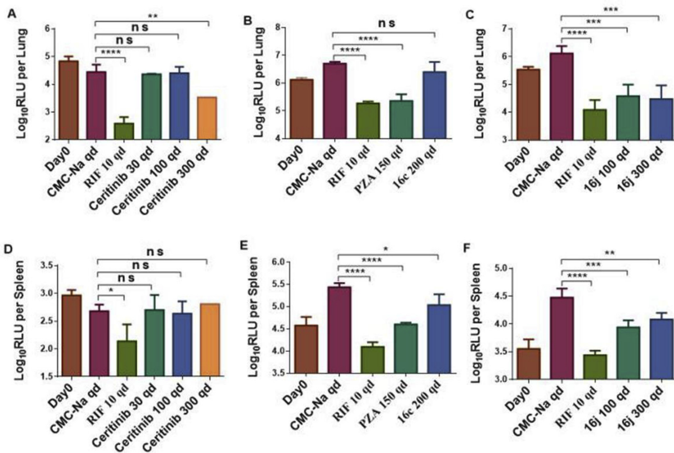
Fig. 2. In vivo efficacy assay showing the lung and spleen bacterial burdens ( \log_{10} RLU) of mice infected with Mtb . Lung (A) and spleen (D) bacterial burdens of mice treated with ceritinib. Lung (B) and spleen (E) bacterial burdens of mice treated with 16c . Lung (C) and spleen (F) bacterial burdens of mice treated with 16j . Mice received treatment for 6 days. Each treatment group comprised four mice. Dosage (mg/kg). Data were presented as mean \pm SD. ns, insignificant; *, P < 0.05 ; **, P < 0.01 ; ***, P < 0.001 ; ****, P < 0.0001 .
