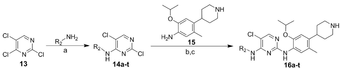
Scheme 3. Reagents and conditions: (a) DIPEA, IPA, 85 °C. (b) HCl, IPA, 85 °C. (c) HCl, ether, rt.
