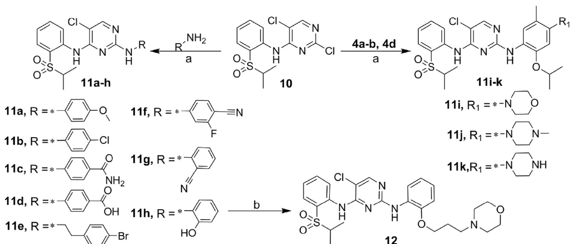
Scheme 2. Reagents and conditions: (a) HCl, IPA, 85 °C. (b) 4-(3-chloropropyl)morpholine, K 2 CO 3 , DMF, 60 °C.
