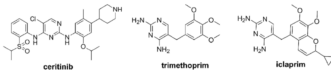
Fig. 1. Chemical structures of ceritinib, trimethoprim, and iclaprim.
