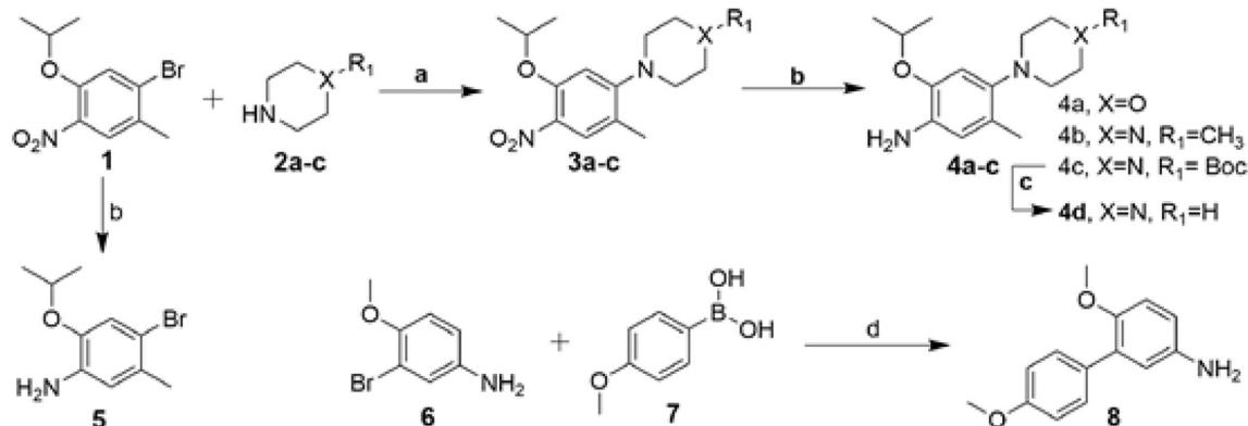
Scheme 1. Reagents and conditions: (a) Pd(AcO) 2 , xantphos, Cs 2 CO 3 , dioxane, 80 °C. (b) Fe, NH 4 Cl, EtOH/H 2 O, 80 °C. (c) TFA, CH 2 Cl 2 , rt. (d) Pd(dppf)Cl 2 , Cs 2 CO 3 , Dioxane, 80 °C.
