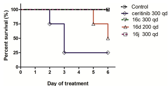
Fig. 3. Percent survival of mice treated with ceritinib, 16c , 16d , or 16j . Mice received treatment for 6 days. Each treatment group comprised four mice. All mice were surveyed for death events. Dosage (mg/kg). Black line + circle, control group; blue line + rhombus, ceritinib group; green line + inverted triangular, 16c group; red line + triangle, 16d group; purple line + square, 16j group. (For interpretation of the references to colour in this figure legend, the reader is referred to the Web version of this article.)
