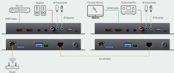
EX-57V3X HDBaseT 3.0 Extender with RS-232, Bi-Directional IR, and USB 2.0
