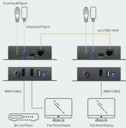
EX-57V3K-M HDBaseT 3.0 Transceiver with RS-232, Bi-Directional IR, and USB 2.0
